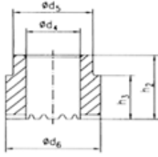
Type RF (for RD type studs)
