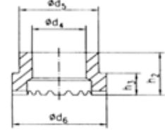
Type RF (for PD type studs) Type UF (for SD, UD, ID type studs)
